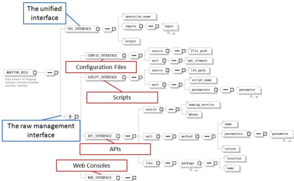
Figure 3. the Mapping Rule for Middleware Management Interfaces
