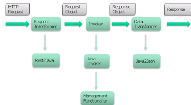
Figure 7. the Approach to JAVA2RESTful
