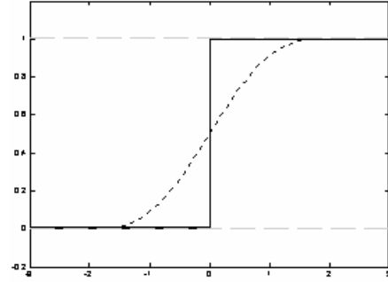
Fig.4. Thickened interface by Heaviside function. Discontinuity (solid line) is smoothed within a “thickness” of \varepsilon=2 .
