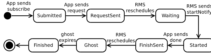
Figure 4: Application states inside the RMS in NDRMSBP.
