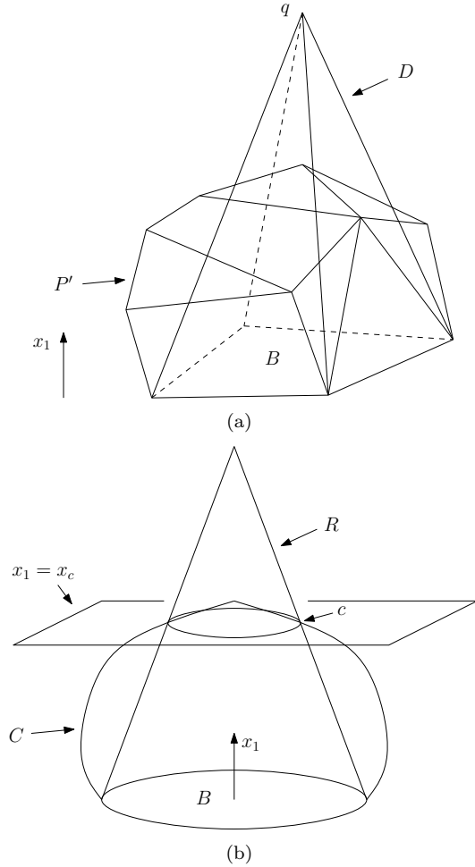
Figure 1: The Schwarz rotation-symmetral of P' and D
