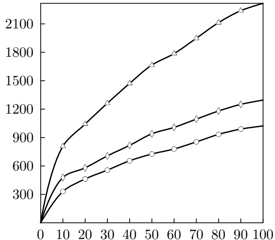
Figure 8: The growth of tree templates. The x axis shows the percentage of the corpus used for extraction, the y axis shows the number of extracted templates ( \triangle ), initial templates ( o ) and auxiliary templates ( \diamond ).
