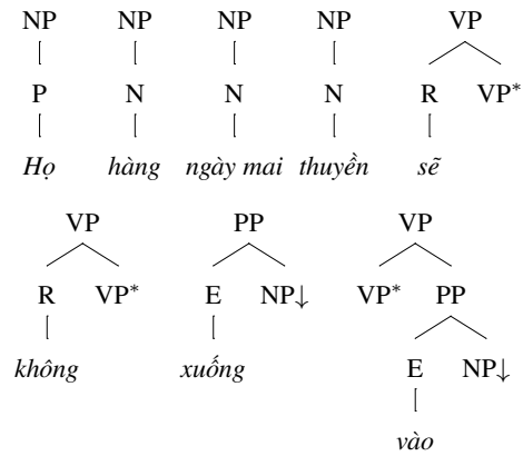
Figure 6: Extracted elementary trees.
