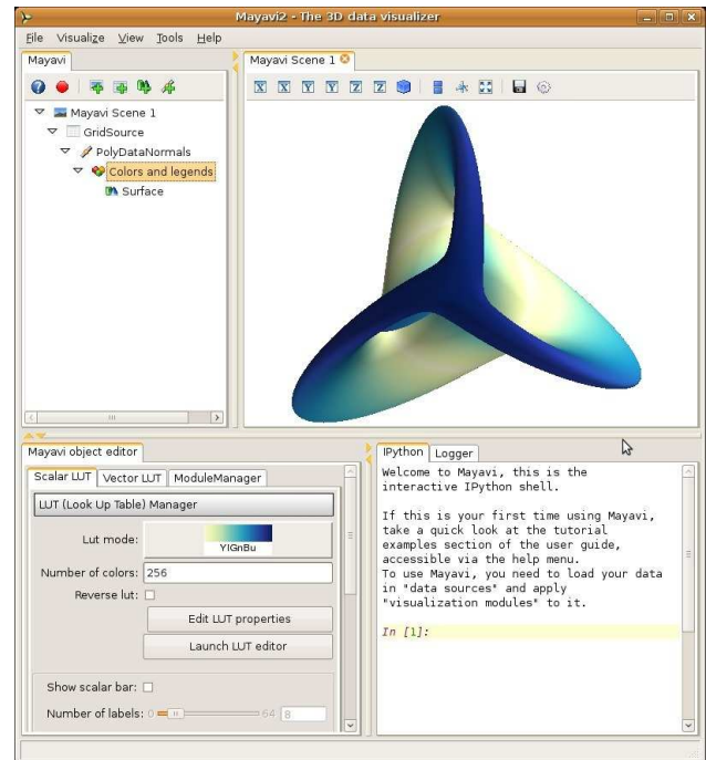
Figure 1: A view of the mayavi2 application showing the Mayavi logo: a Boy mathematical surface. On the bottom right, an interactive IPython prompt, for prototyping scripts or exploring objects, can be seen. On the upper left stands the tree representing the visualization pipeline. It features a source, here a grid of points created by numpy arrays, a PolyDataNormal filter used to calculate normals of the surface for a smooth rendering, and the Surface module, with its corresponding module-manager node, used to change the colors and legend of the surface. The dialog below the tree can be used to modify the selected node, i.e. colors and legend properties in the present case.
