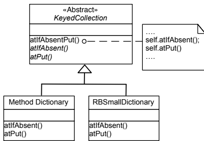
Figure 7: Template Method represented in concept c_7 of the class hierarchy example
