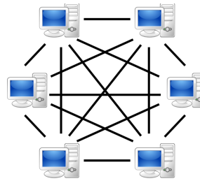
Figure 1: peer-to-peer architecture
