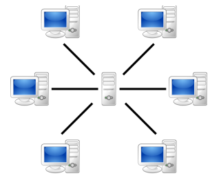
Figure 2: client/server architecture
