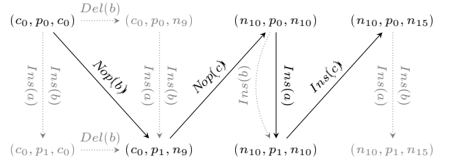
Figure 8: The propagation graph G_{n_6} .
