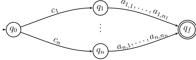
Fig. 5. Illustration of a fragment of the constructed automaton M in the proof of Lemma 11.
