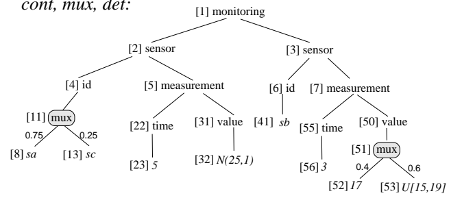
Figure 6: \text{PrXML}^{\text{cont}, \text{mux}, \text{det}} p-document: monitoring.
