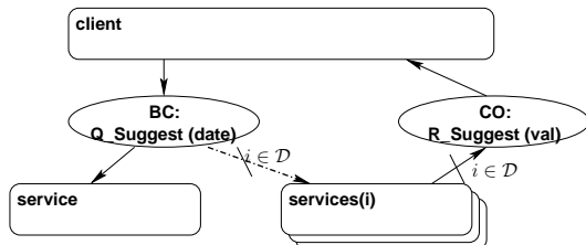
Figure 1. Graphical representation of broadcasting operator
