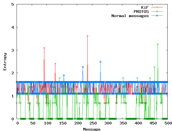
Fig. 9. Entropy for two fuzzers on SJphone.
