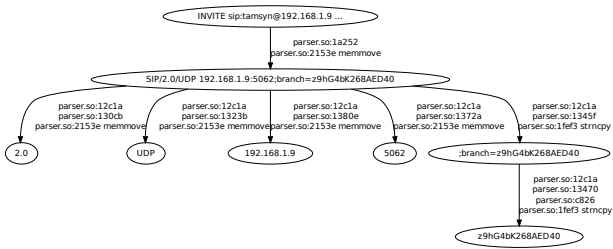
Fig. 2. Simple parsing example.
