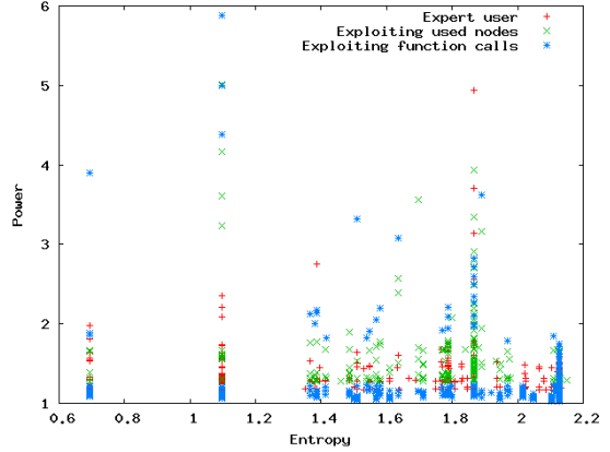
Fig. 16. Lighttpd: power vs entropy
