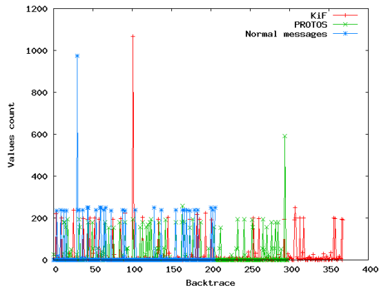
Fig. 3. Coverage of different fuzzers on Linphone.
