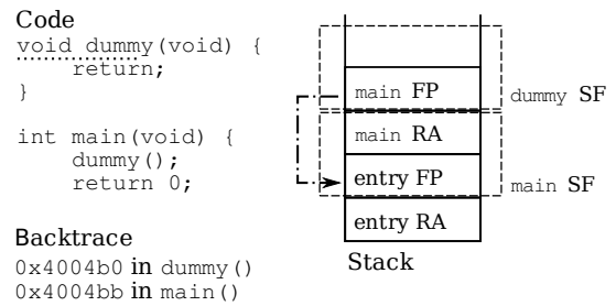
Fig. 1. Example of a simple backtrace.
