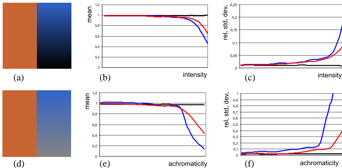
Fig. 4. a,d) frame from test sequence with constant optical fbw of one pixel per frame. b,c) mean and relative standard deviation mean of the optical fbw based on RGB (black line), shadow-shading invariant (blue line) and robust shadow-shading invariant (red line). e,f) mean and relative standard deviation of the optical fbw based on RGB (black line), shadow-shading-specular invariant (blue line) and robust shadow-shading-specular invariant (red line).
