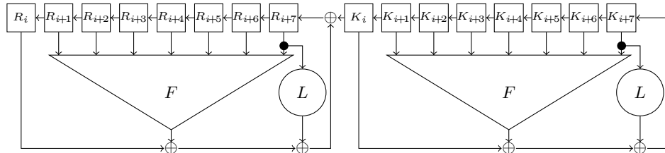
Fig. 2. ESSENCE Round Function (iterated 32 times).
