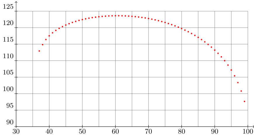
Fig. 4. Distribution of the number of carries in rounds 19–50 of XTEA. \log_2 of the number of keys with a given number of carries. 48% of the keys have less than 60 carries, and 52% have less than 61 carries.
