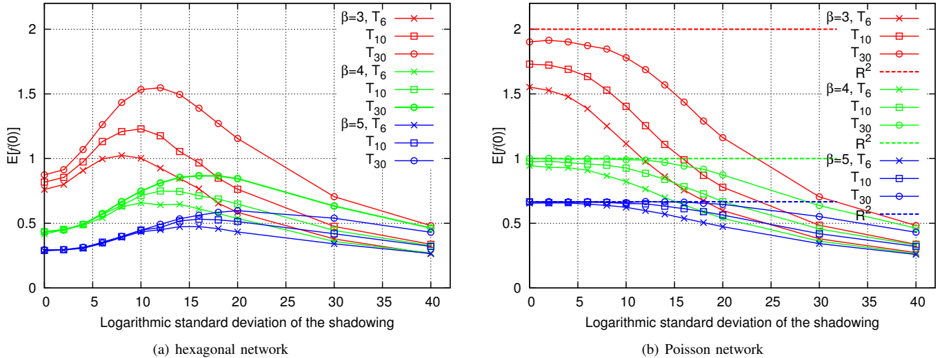
Fig. 4. Mean interference factor in hexagonal and Poisson network on the torus \mathbb{T}_N with log-normal shadowing with log-SD v and path-loss exponent \beta . Note that \mathbf{E}[f(0)] increases with the size of the network. The straight lines correspond to the infinite (on \mathbb{R}^2 ) Poisson model; cf. Proposition 5.6.
