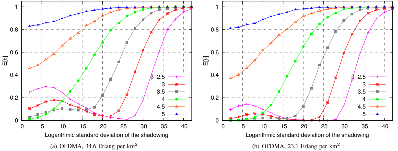
Fig. 3. Blocking probability for OFDMA network as on Figure 2 with traffic 34.6 Erlang per km 2 and 23.1 Erlang per km 2 .
