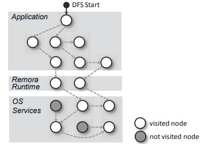
FIGURE 13. Using depth-first search algorithm to discover the orphan nodes.
