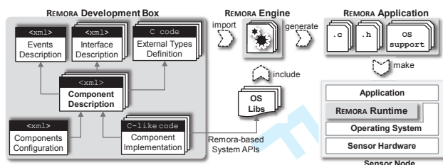
FIGURE 10. REMORA-based development process.
