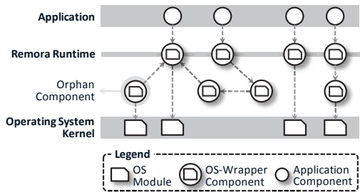
FIGURE 12. The REMORA engine tunes the operating system by tracing component dependencies and finding orphan components.
