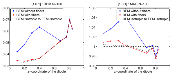
Fig. 4. Comparison of BEM to the FEM with the fiber for dipoles oriented [1, 0, 1] . RDM (left), MAG (right).
