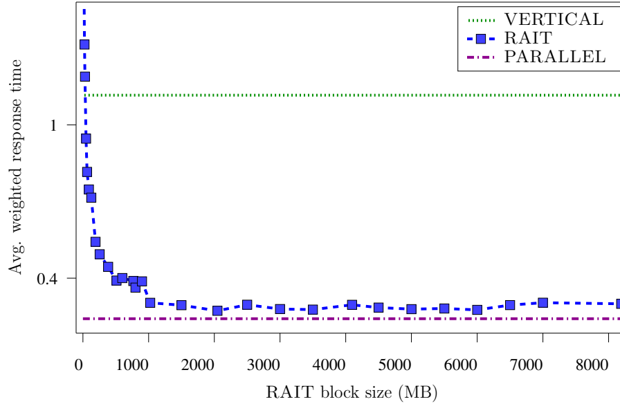
Figure 5: Impact of RAIT block size B on average weighted response time.
