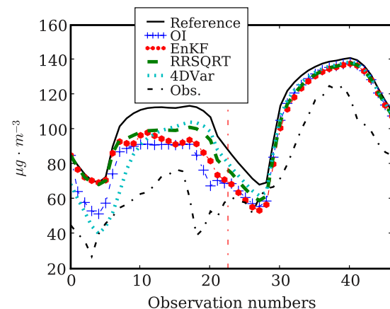
Figure 5. Time evolution of ozone forecasts against available observations over 2 days at EMEP station Montandon.
