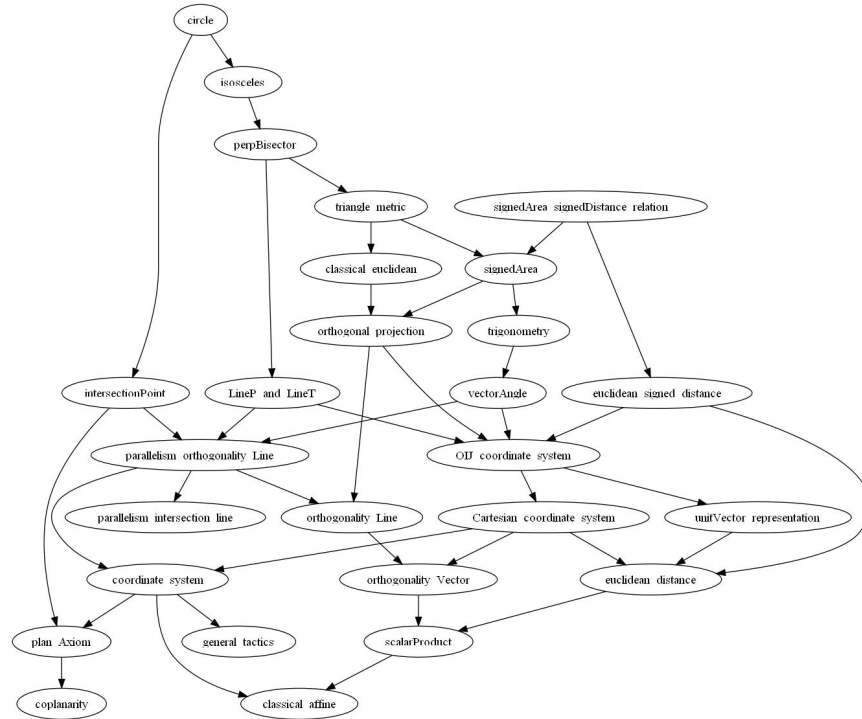
Fig. 2: Formalization of plane geometry
