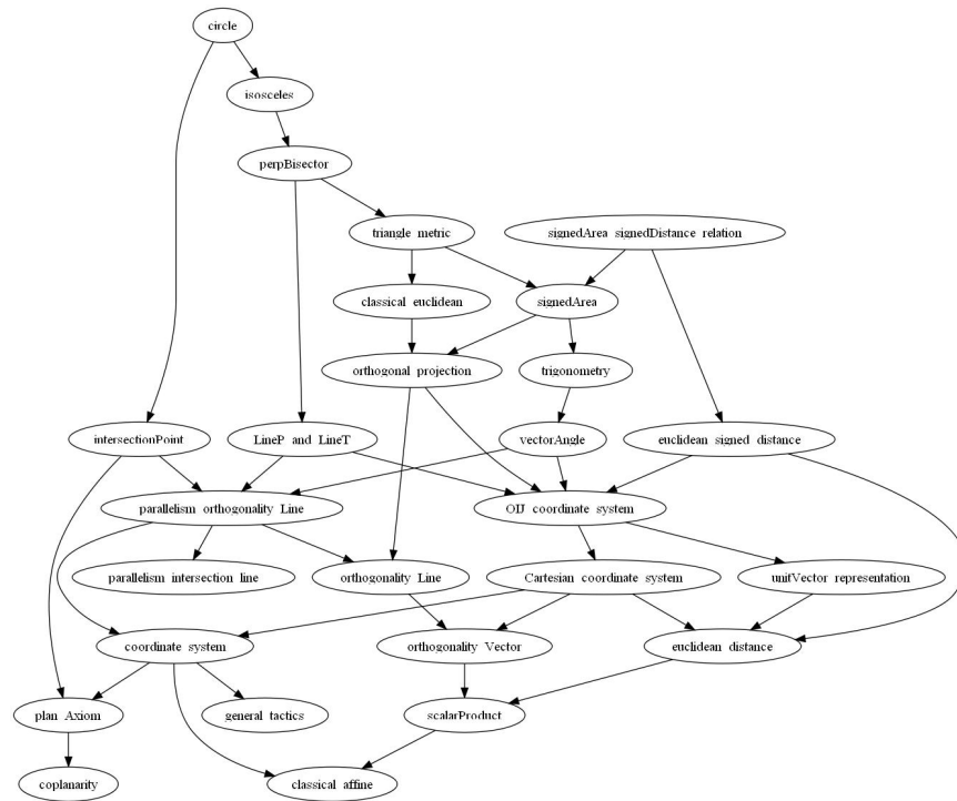
Fig. 2: Formalization of plane geometry
