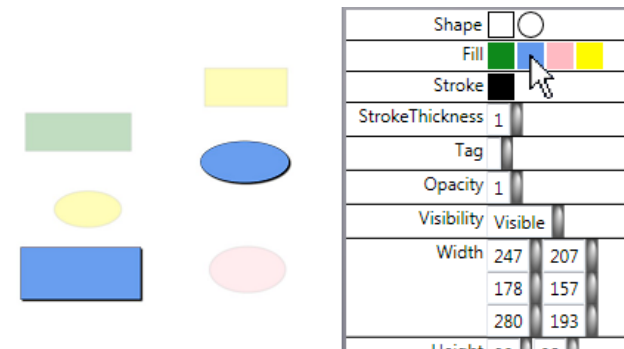
figure 3. The user's cursor is over the blue shared value of the fill property (fill: blue). Because they don't have this shared value, the green rectangle, the pink circle and the two yellow shapes are dimmed.
