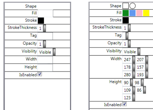
figure 2. The user's selection contains objects with varying shapes, fill colors, width, and height. A classical property sheet (left) displays a blank fill for those properties, whereas our property sheet (at right) displays all different values.
