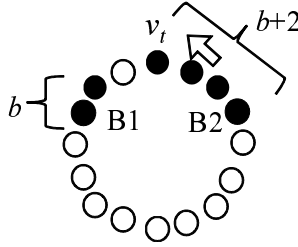
Figure 5: Semi-twin C_{st}(b)
