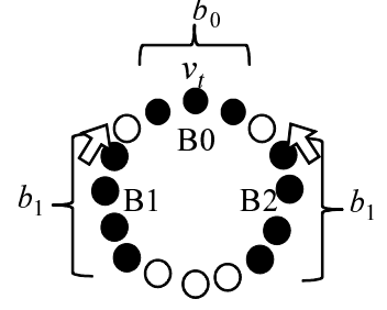
Figure 3: Block leader C_{bl}(b_0, b_1)
