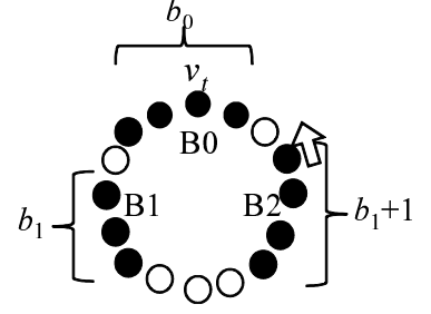
Figure 6: Semi-block leader C_{sbl}(b_0, b_1)
