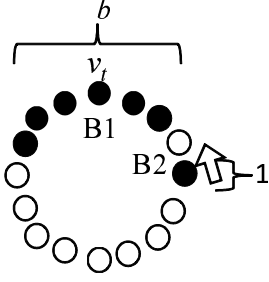
Figure 4: Semi-single block C_{ssb}(b)
