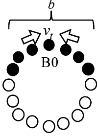
Figure 1: Single block C_{sb}(b) ( b > 2 )
