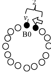
Figure 2: Single block C_{sb}(2)
