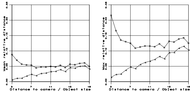
Fig. 4. The behaviour of the factorization method (small squares) is compared with the behaviour of the iterative method described in this paper (small triangles) as a function of the relative distance between the object and the camera (see text). The left side shows the mean value of the distance between object points and reconstructed points and the right side shows the maximum value of this distance.
