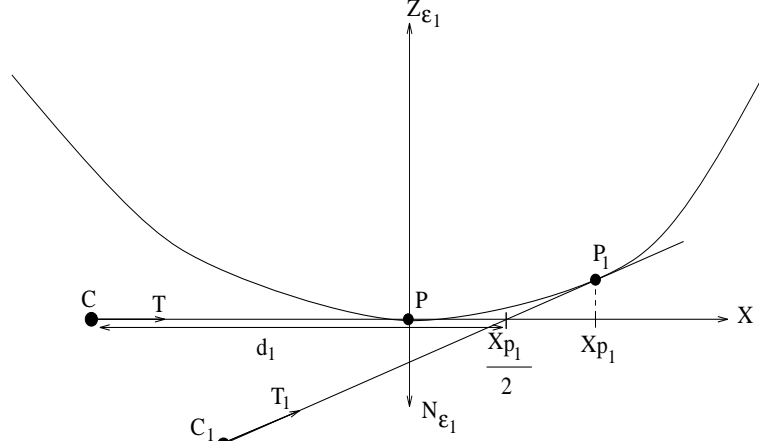
Figure 6: The epipolar plane \mathcal{E}_1 .
