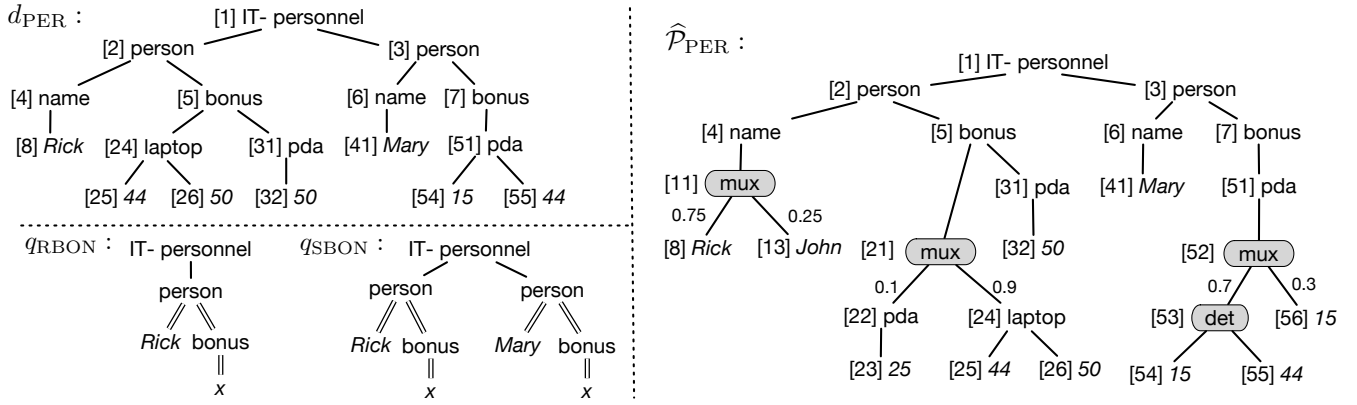
Figure 1: Example p-document \hat{\mathcal{P}}_{\text{PER}} , possible document d_{\text{PER}} of \hat{\mathcal{P}}_{\text{PER}} , TP query q_{\text{RBON}} and TPJ query q_{\text{SBON}}
