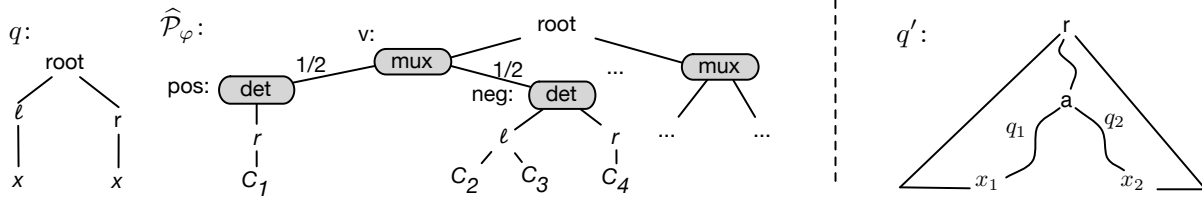
Figure 3: For Theorem 15. Left: a TPJ query q with an essential join and a p-document \widehat{\mathcal{P}}_\varphi encoding \varphi = (w_1 \wedge v) \vee (\neg v \wedge w_2) \vee (\neg v \wedge w_3) \vee (w_4 \wedge \neg v) . Right: a general pattern q' of a TPJ query with an essential join.
