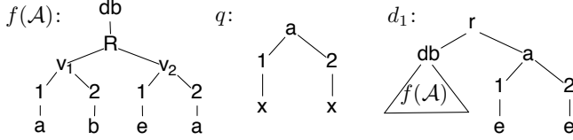
Figure 2: Left: translation from a finite relational structure \mathcal{A} = \{R(a, b), R(e, a)\} into a tree f(\mathcal{A}) (Lemma 10). Center: a TPJ query with an essential join (Theorem 11). Right: a document d (Theorem 11).
