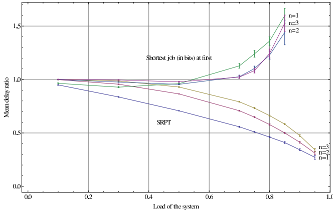
Fig. 3. Mean delay of SRPT and modified SRPT compared with PS as a function of the load of the system with 95 % confidence interwalls.
