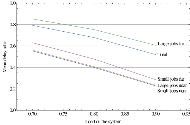
Fig. 6. Relative performance improvement of SRPT compared to PS for the conditional mean delays.
