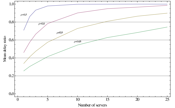
Fig. 2. The effect of n = K/k on the performance improvement of SRPT.
