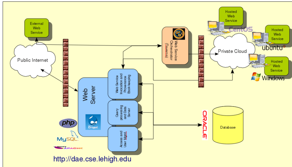
Figure 1. Overview of the DAE platform architecture
