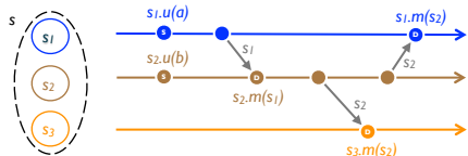
Figure 1: State-based replication
