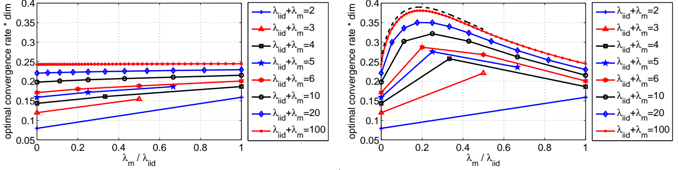
Figure 3: Optimal asymptotic convergence rates CR^{\text{opt},\infty}(\lambda_{\text{iid}}, \lambda_m) , Equation (24), for the (\mu/\mu_w, \lambda_{\text{iid}} + \lambda_m) -ES versus the ratio \lambda_m/\lambda_{\text{iid}} of mirrored and independent offspring for various \lambda = \lambda_{\text{iid}} + \lambda_m . Left: (\mu/\mu_w, \lambda_{\text{iid}} + \lambda_m^{\text{rand}}) -ES with random mirroring. Right: (\mu/\mu_w, \lambda_{\text{iid}} + \lambda_m^{\text{sel}}) -ES with selective mirroring, mirroring the worst \lambda_m from \lambda_{\text{iid}} independent offspring. In addition, the righthand plot shows the theoretical result for \lambda_{\text{iid}} \rightarrow \infty of Equation (25) as a dashed line.
