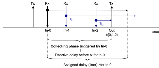
Figure 4: Collecting phase of a node participating in flooding.
