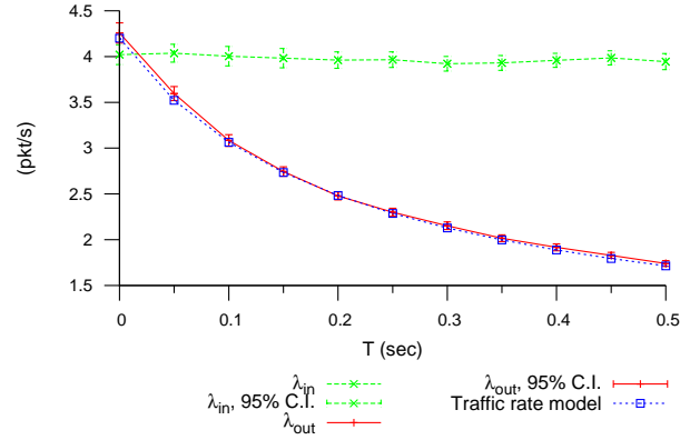
Figure 8: Out-packet ( \lambda_{out} ) and in-packet ( \lambda_{in} ) rates, for different values of T , and a theoretical in-packet rate \lambda_{in} = 4 \frac{pkt}{s} (simulations and analytical results).
