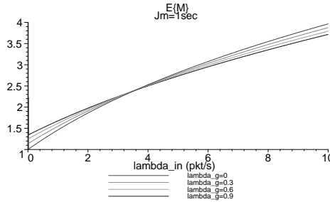
Figure 5: Mean of M depending on \lambda_{in} , for different values of \lambda_g , J_m = 1sec .
