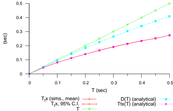
Figure 7: Average time to transmission for \lambda_{in} = 4 \frac{pkt}{s} , \lambda_g = 0.2 \frac{pkt}{s} , for different values of t (simulations and analytical results).
