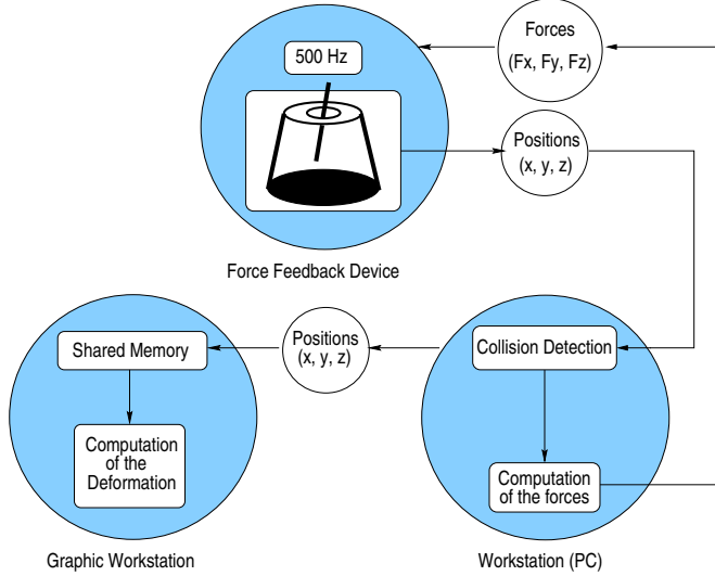
Figure 6: Example of simulation systems.
