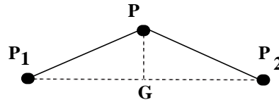
Figure 3: Geometric definition of local regularity.
