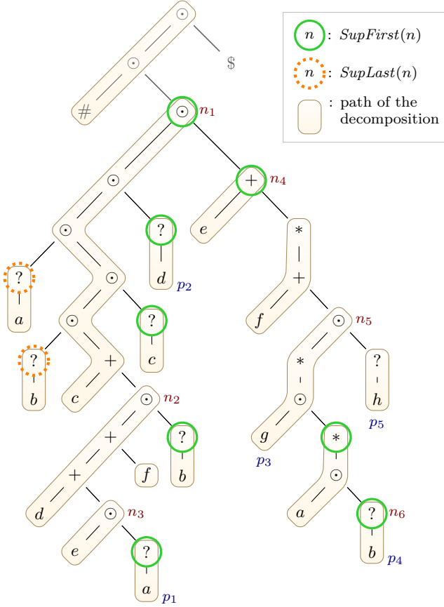
Figure 2: Path decomposition.
