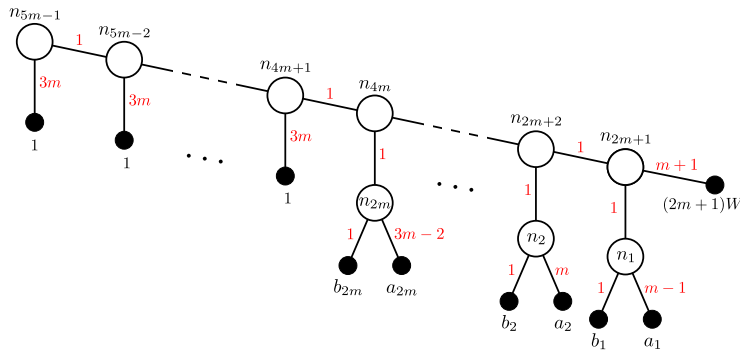
Figure 5: Instance \mathcal{I}_6 .
