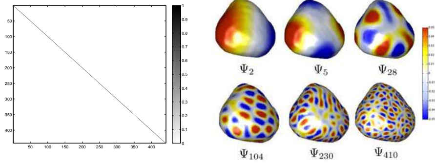
Fig. 3. Left: inner products of eigenfunctions of the Laplacian for every pairs [15]. The pairs are rearranged from low to high degree. Right: representative eigenfunctions \Psi_j on the left amygdala template surface obtained by solving \Delta\Psi_j + \lambda_j\Psi_j = 0 .
