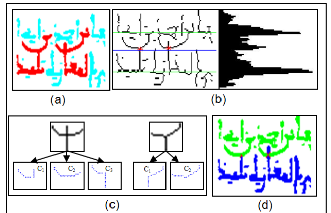
Fig. 15 Different steps of the separation of connected components.
