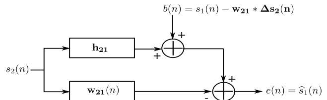
Figure 2: Equivalent adaptive plant identification of \mathbf{h}_{21} . On this scheme, \Delta \mathbf{s}_2(n) denotes the vector composed of artifact signals and defined by \Delta s_2(n) = \hat{s}_2(n) - s_2(n) .
