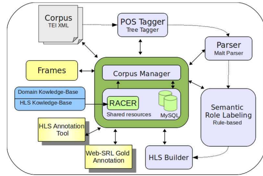
Figure 2: General Architecture for the HLS Annotation.
