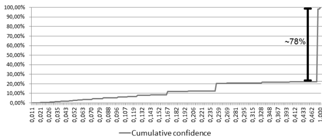
Figure 8. Cumulative confidence
