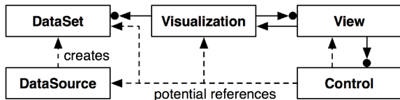
Figure 1: The Information Visualization Reference Model [24]
