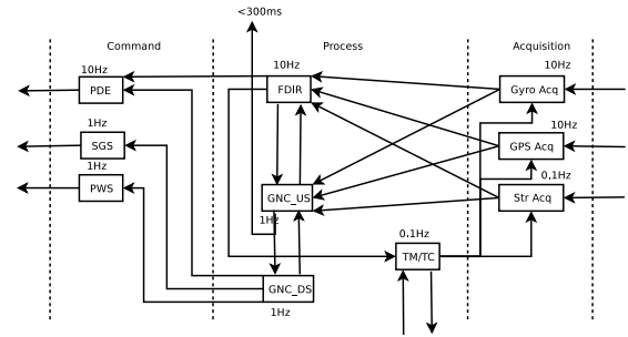
(a) The Flight Application Software
